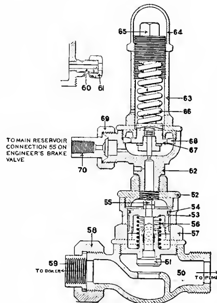
Fig. 1716. WESTINGHOUSE PUMP GOVERNOR.
